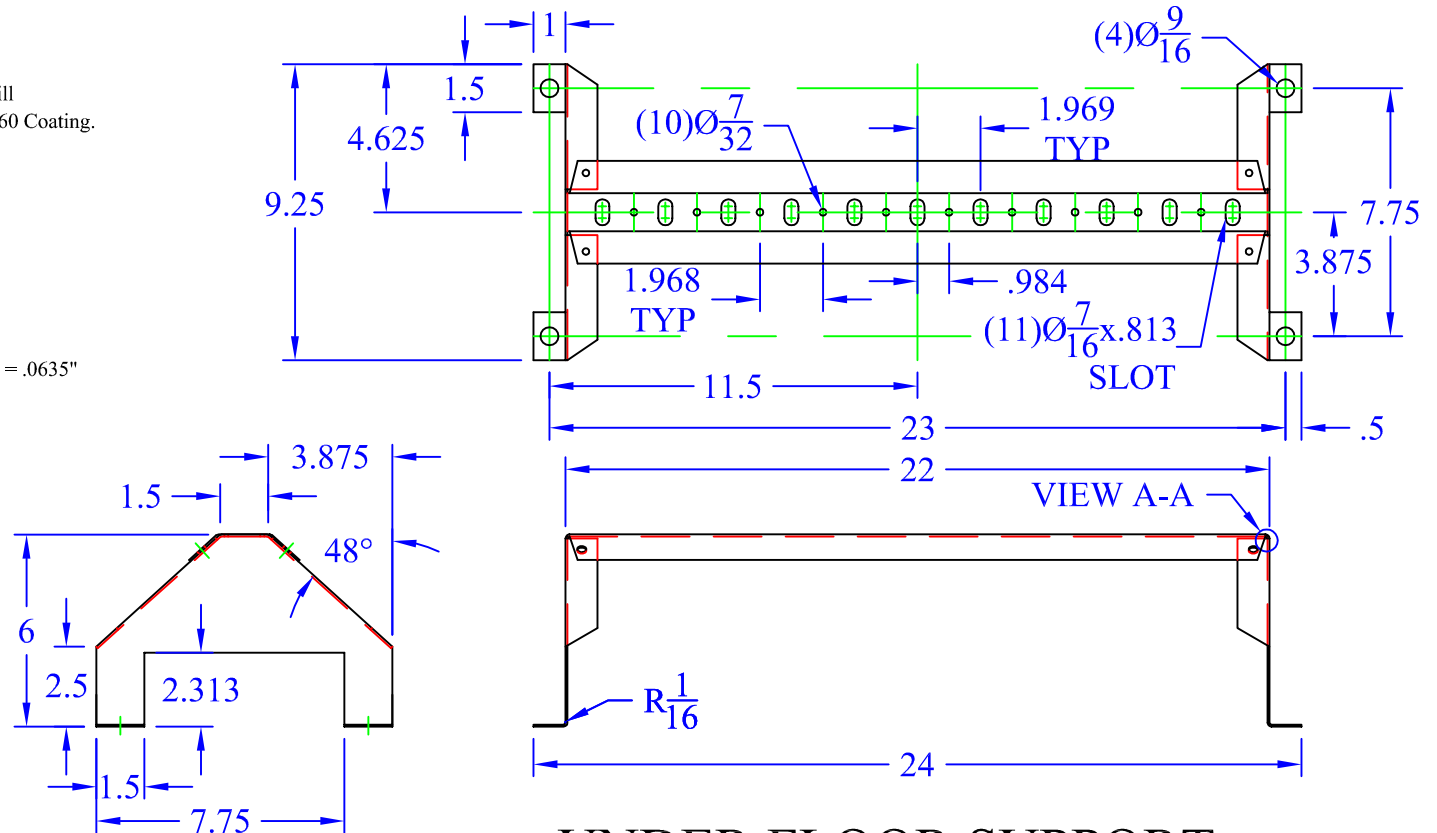
UNDER FLOOR SUPPORT SCALE: 2"=1'
