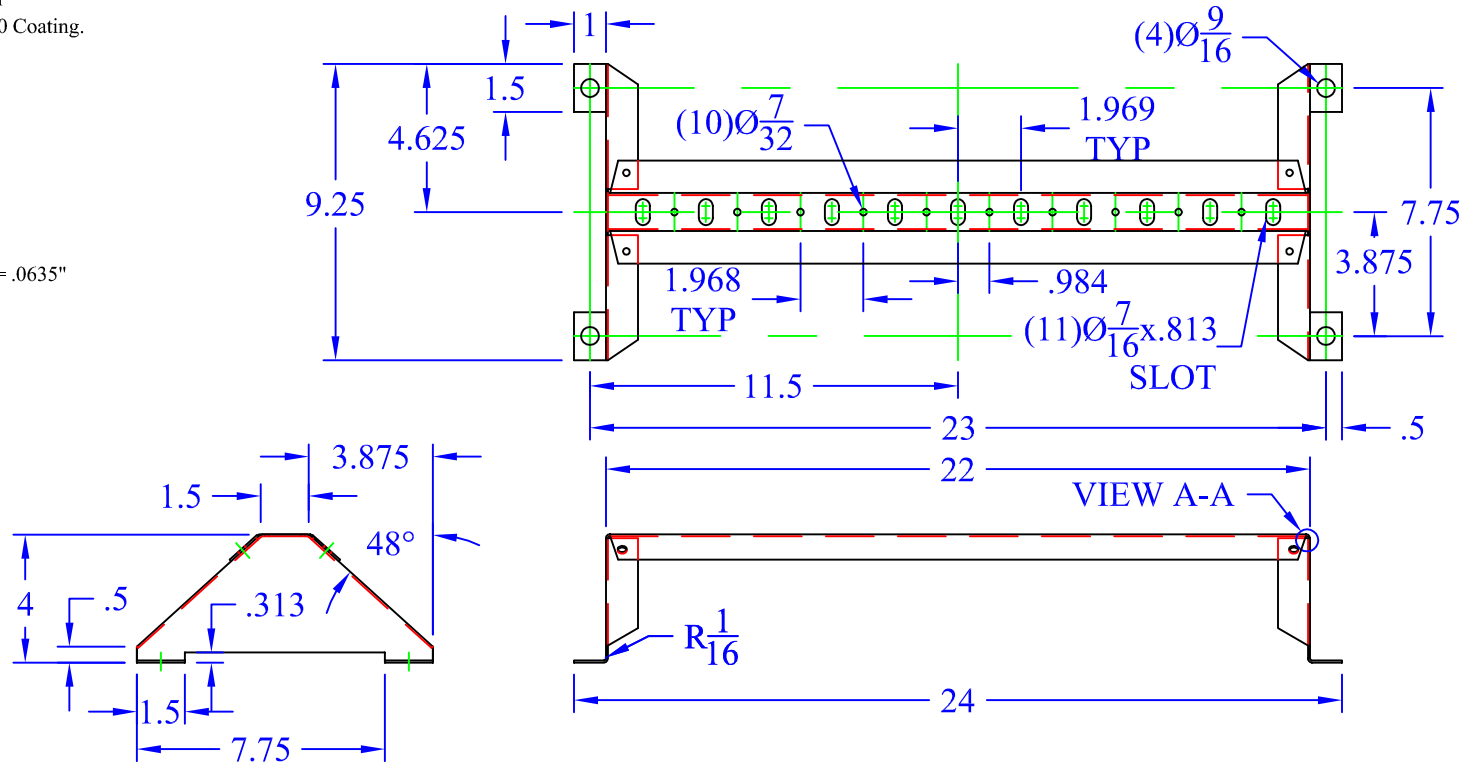
UNDER FLOOR SUPPORT SCALE: 2"=1'
