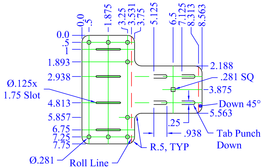
Flat Pattern View
