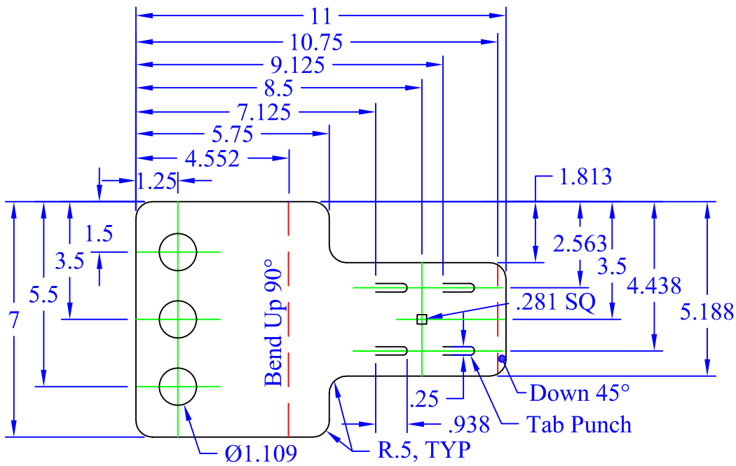
Flat Pattern View
