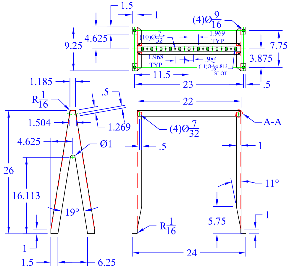
FLOOR SUPPORT SCALE: 1"=1'
