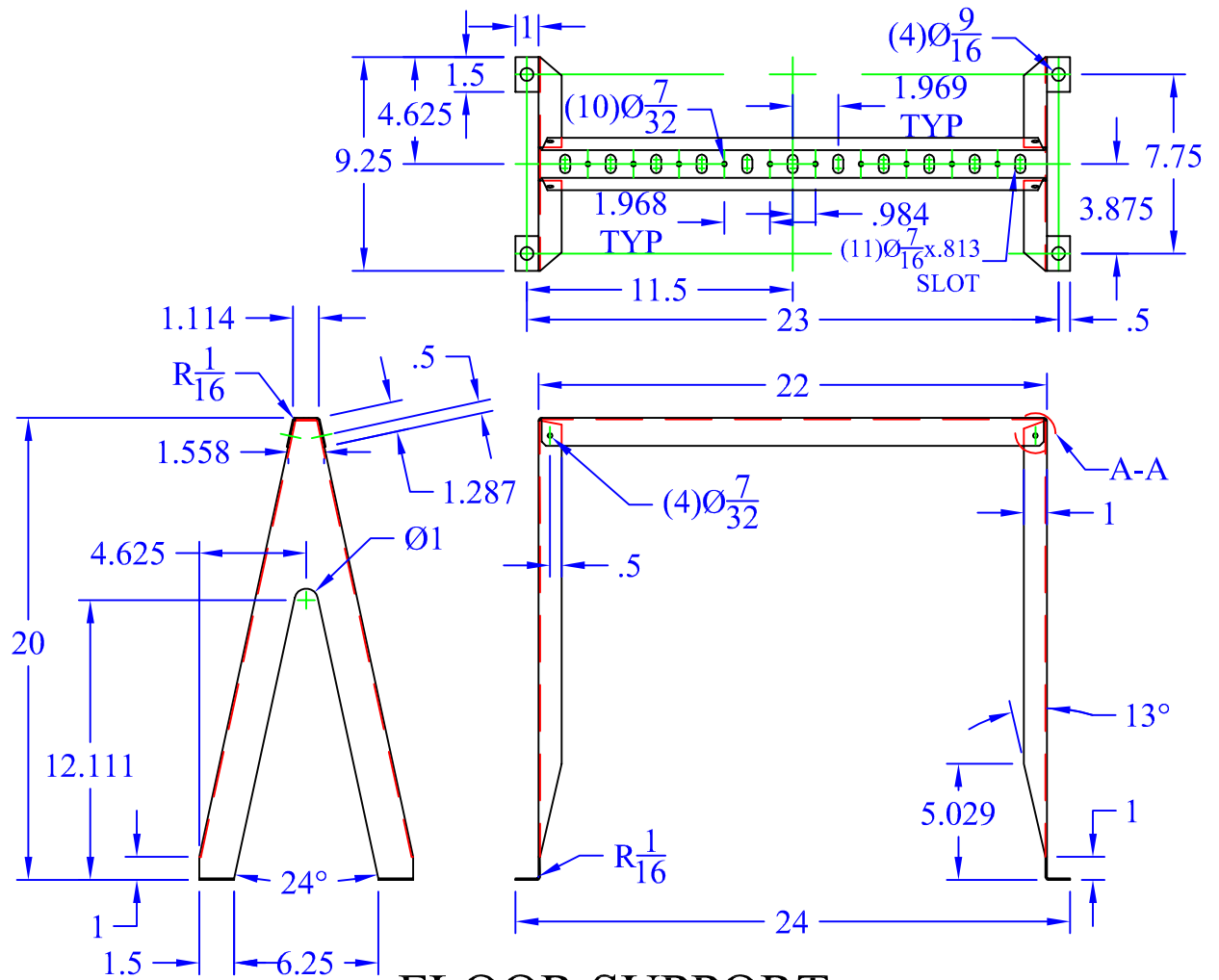
FLOOR SUPPORT SCALE: 1-1/2"=1'
