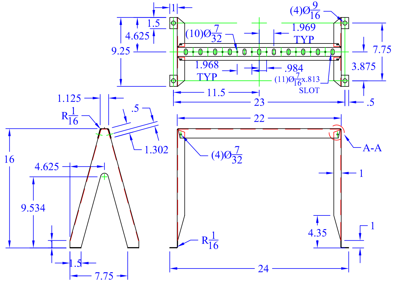
FLOOR SUPPORT SCALE: 1-1/2"=1'
