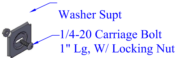
(6) Washer Supt
