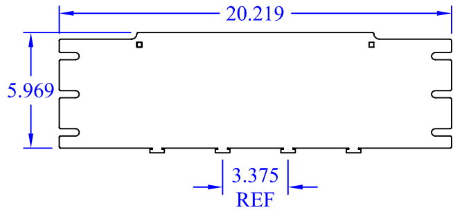
(1) WBT-T-6x4 TBACK
