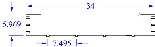
(1) WBT-T-6x18 TBACK
