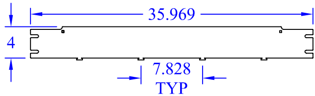
(1) WBT-T-4x20 TBACK
