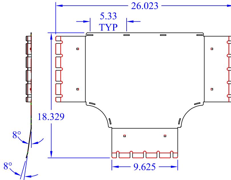
(1) WBT-T-Xx10 BASE
