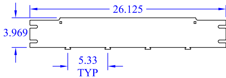
(1) WBT-T-4x10 TBACK
