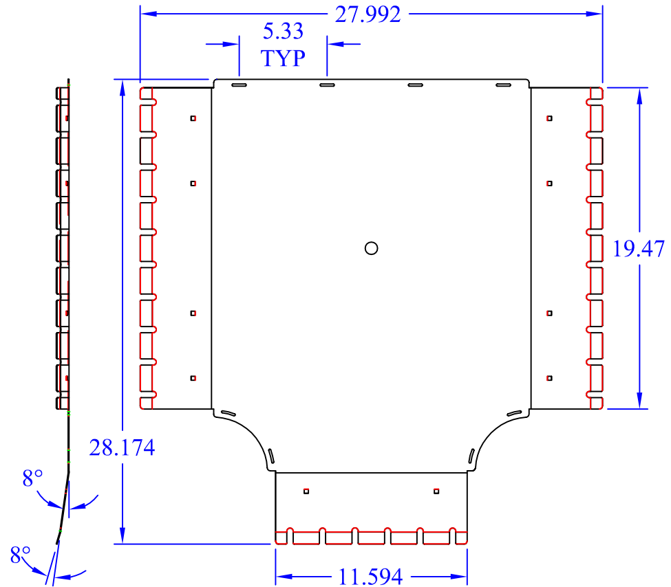
(1) WBT-T-Xx20-12PG BASE
