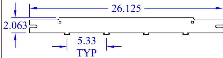
(1) WBT-T-2x10 TBACK
