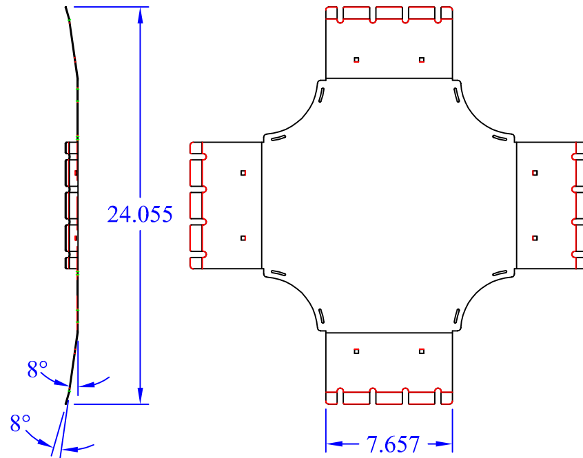
(1) WBT-I-Xx8 Base
