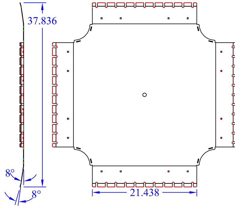
(1) WBT-I-Xx22 Base
