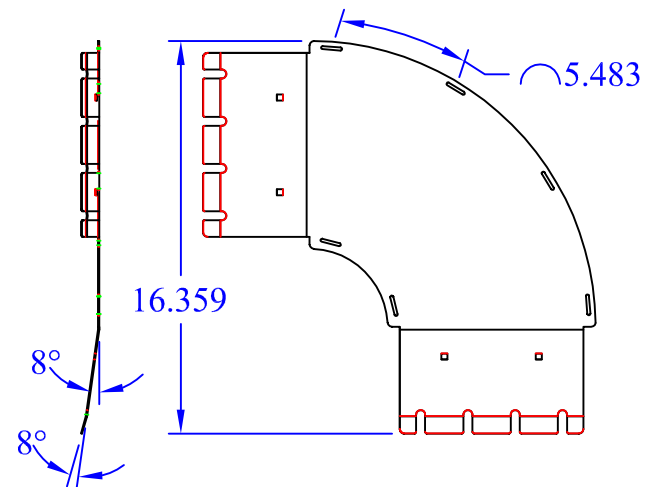
(1) WBT-90-Xx8 Base
