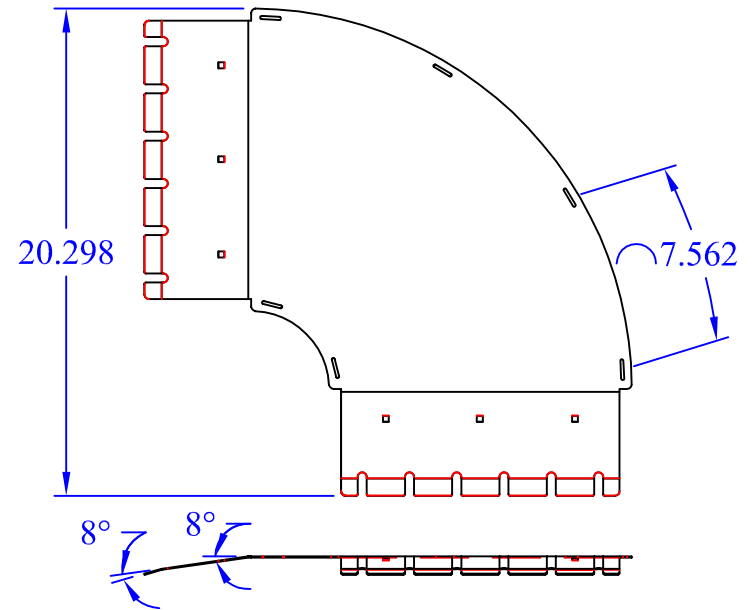
(1) WBT-90-Xx12 Base
