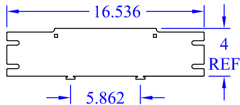
(1) WBT-45-4x6 OR
