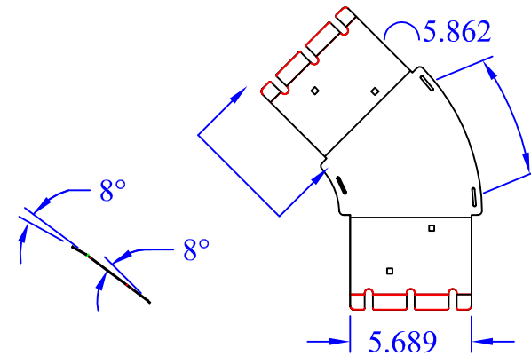
(1) WBT-45-Xx6 Base
