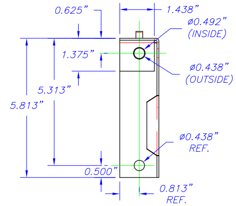
DETAIL B-B
