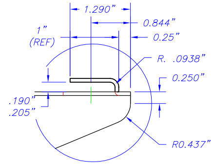
HOOK AND END DETAIL C-C
