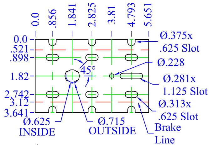
Flat Pattern Layout
