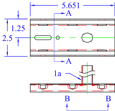
Formed Layout View
