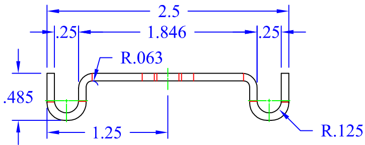
View A-A 1"=1"
