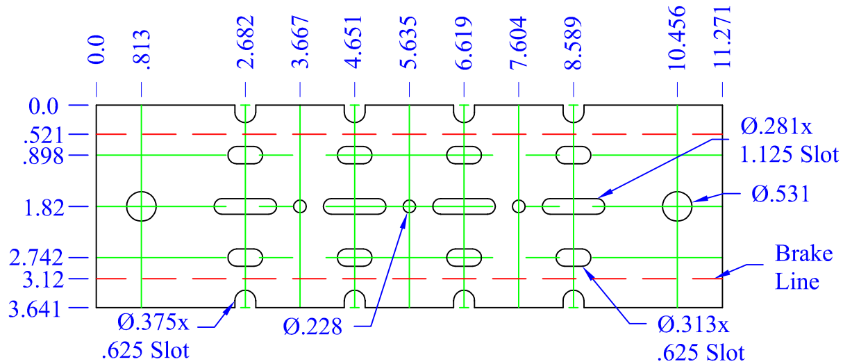
Flat Pattern View
