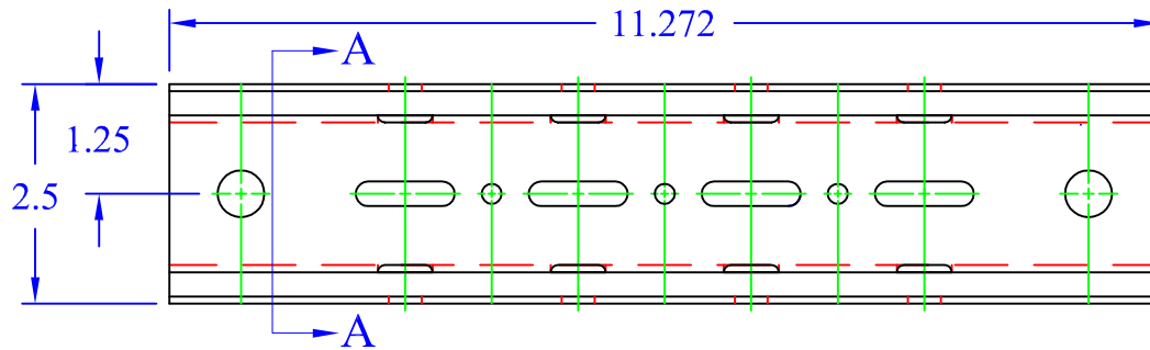
Formed View
