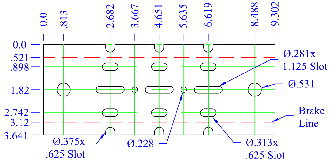
Flat Pattern View
