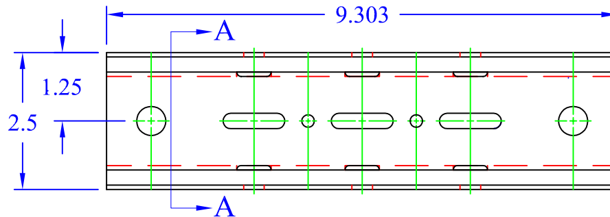
Formed View
