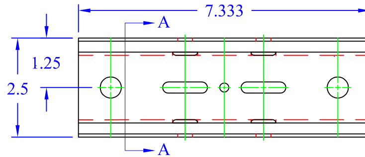
Formed View
