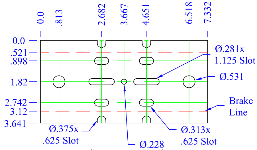
Flat Pattern View
