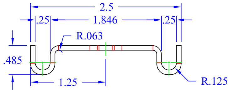
View A-A 1"=1"
