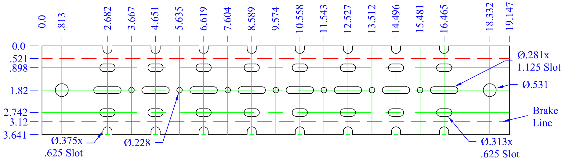
Flat Pattern View
