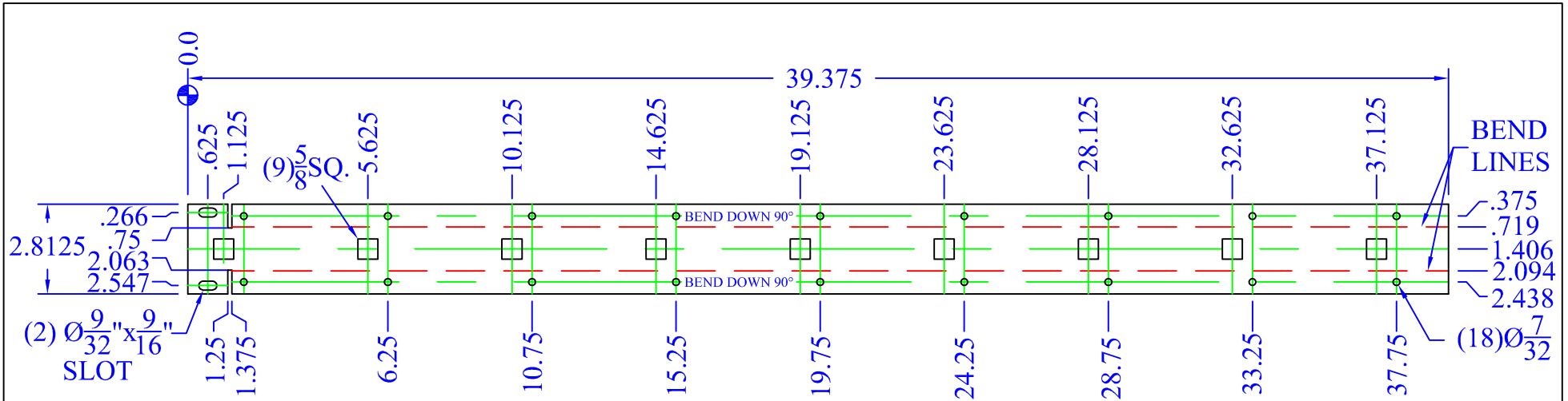
Flat Layout Plan View
