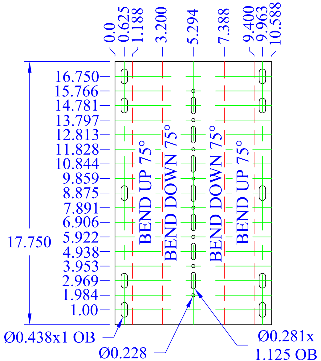
FLAT LAYOUT PLAN
