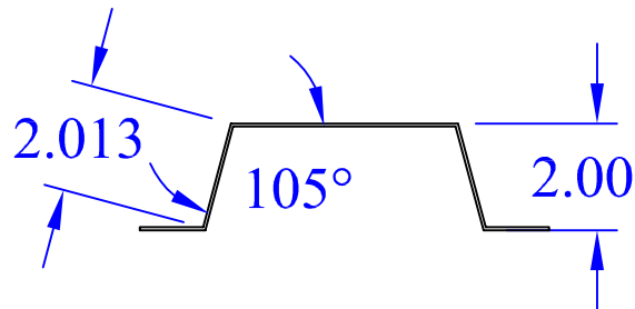
BENT VIEW
