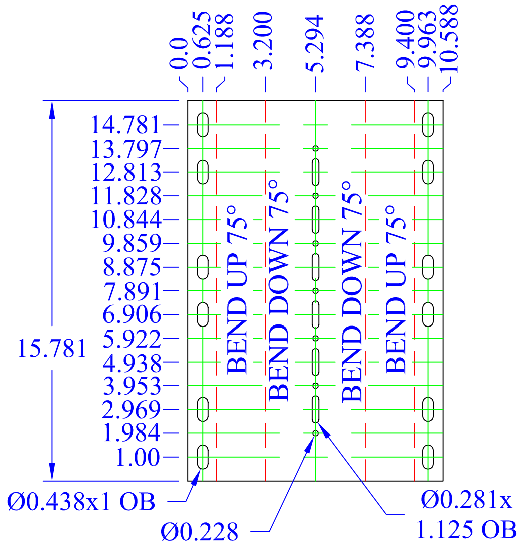
FLAT LAYOUT PLAN
