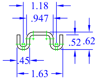
VIEW A-A 6"=1'
